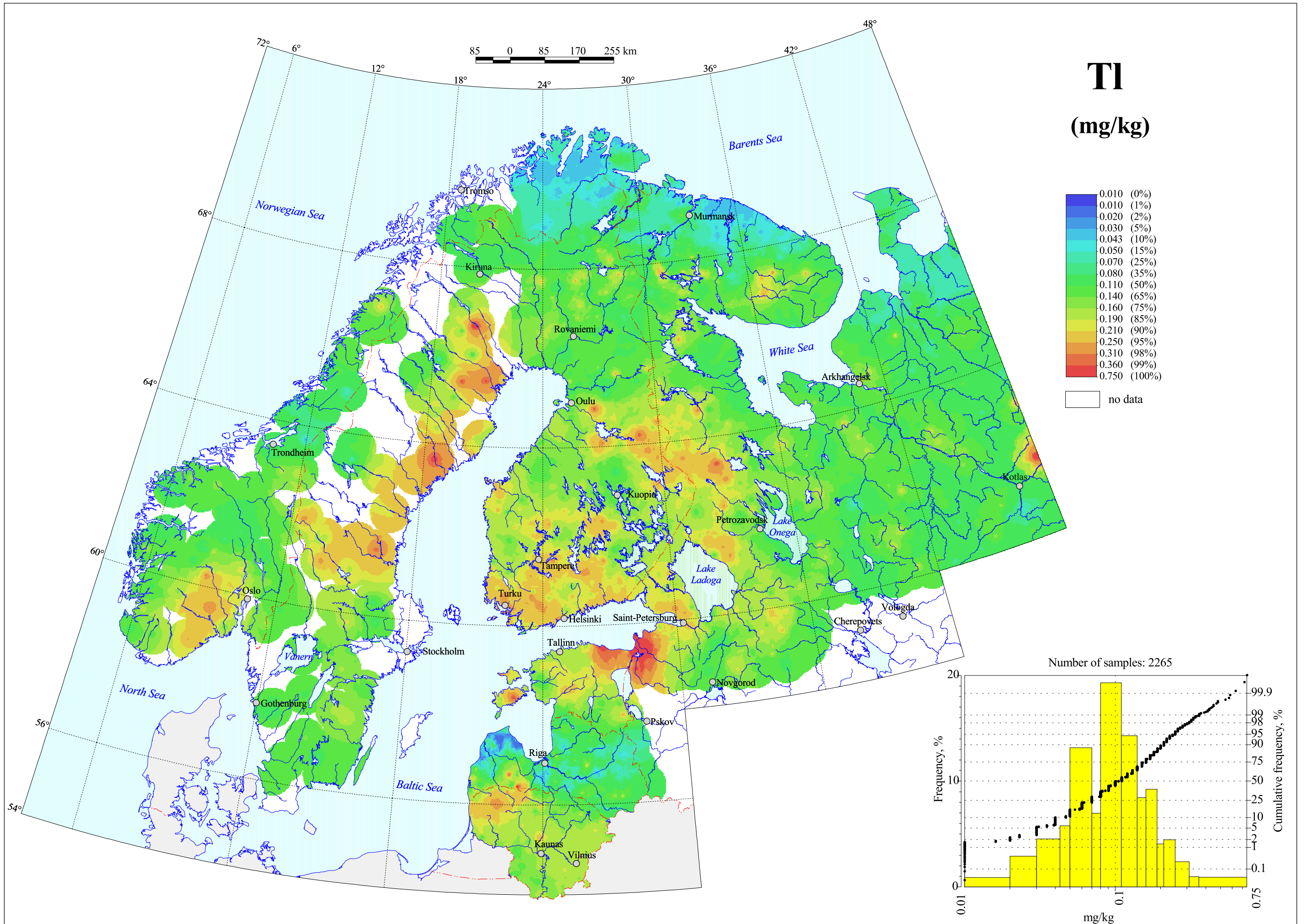
Thallium in Organic Soil Layer, Total Content
